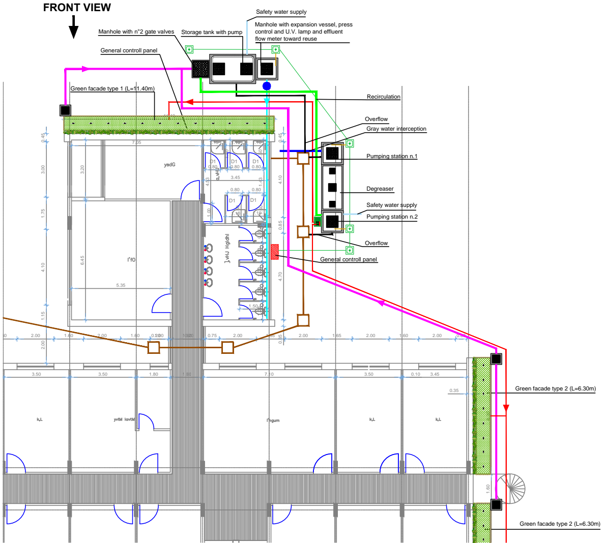
Green Facade plan (Area 1, 2, 3)
